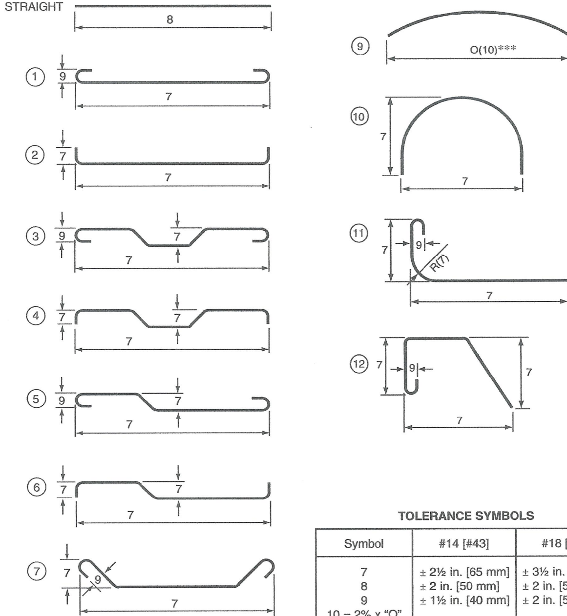
FIGURE 7-4 STANDARD FABRICATING TOLERANCES—ACI 315 For bar sizes #14 and #18 [#43 and #57]
