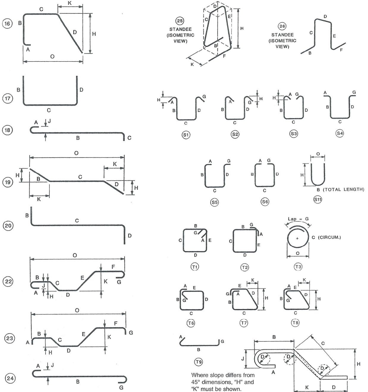
FIGURE 6-2 TYPICAL BAR BENDS (CONT.)
