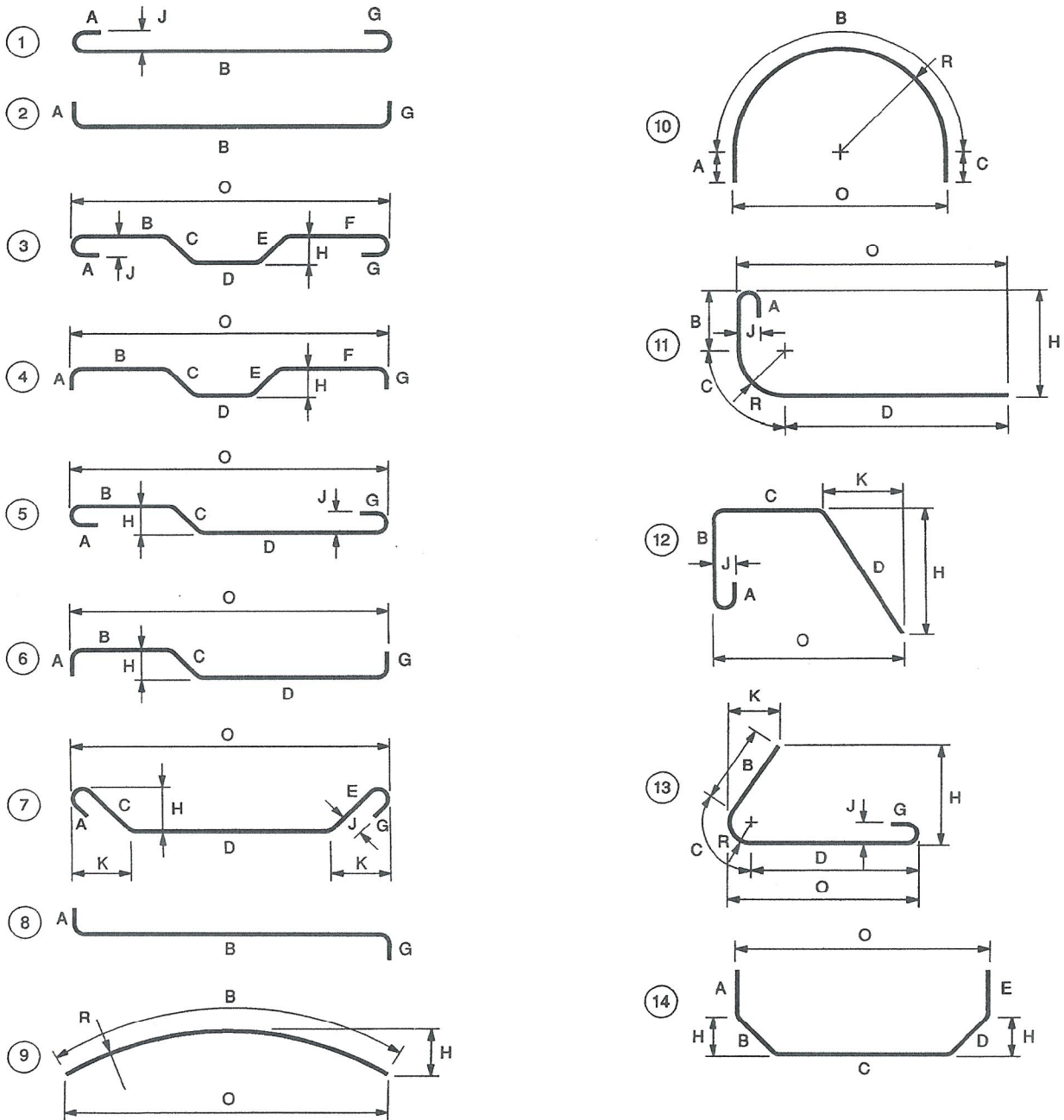
FIGURE 6-2 TYPICAL BAR BENDS
